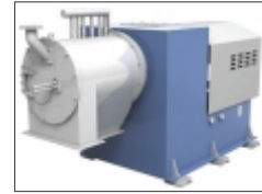
Pusher Centrifuge
